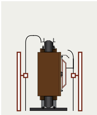
Bottom cabling (Cable)
